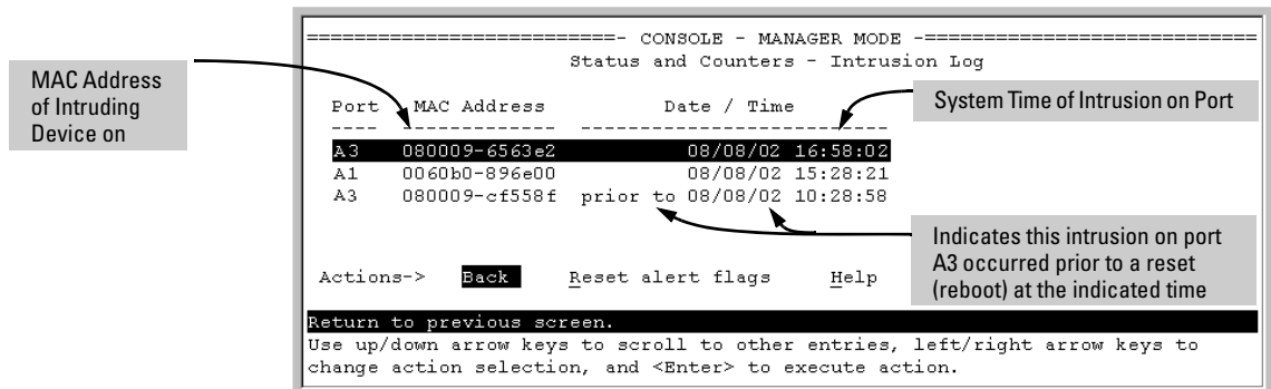
Figure 13-14. Example of the Intrusion Log Display
